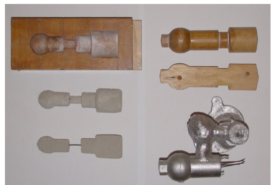
Wooden patterns are made to cast Aluminium
