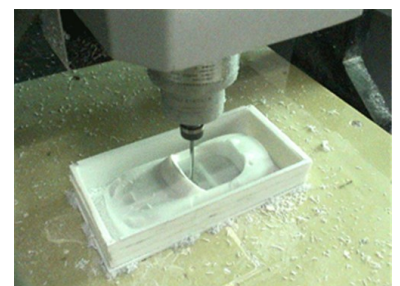
CNC 3D Milling machine cutting out a profile for a model car
